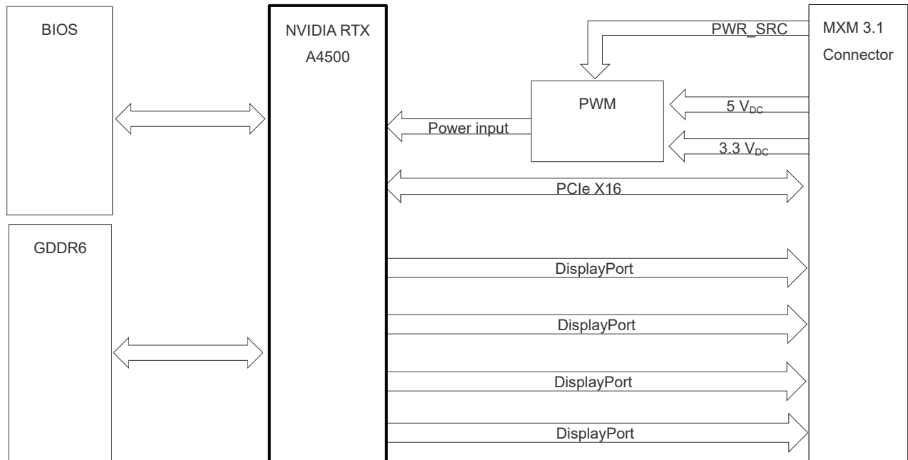
M3A4500-WP Block diagram
