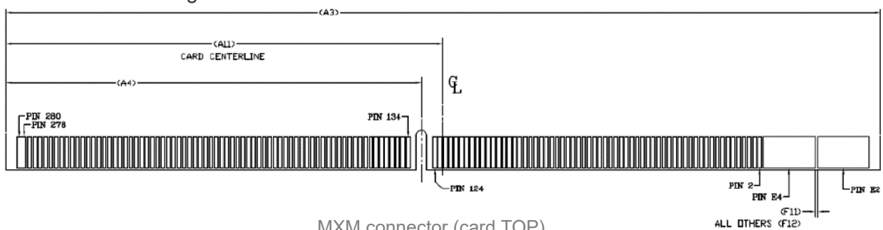
MXM connector (card TOP)
