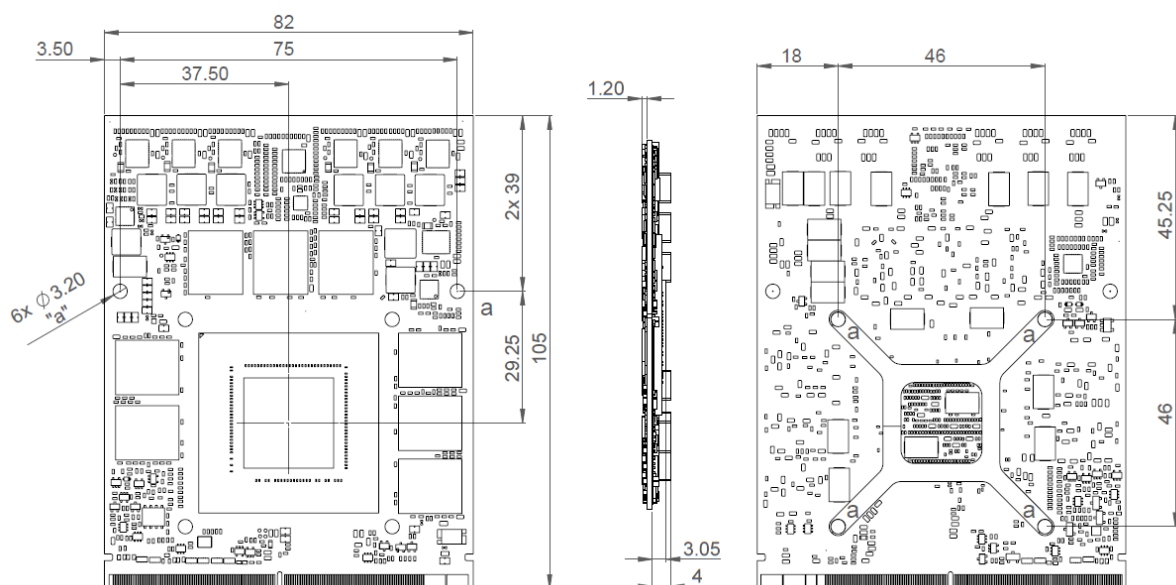
Dimensions of M3A4500-WP
